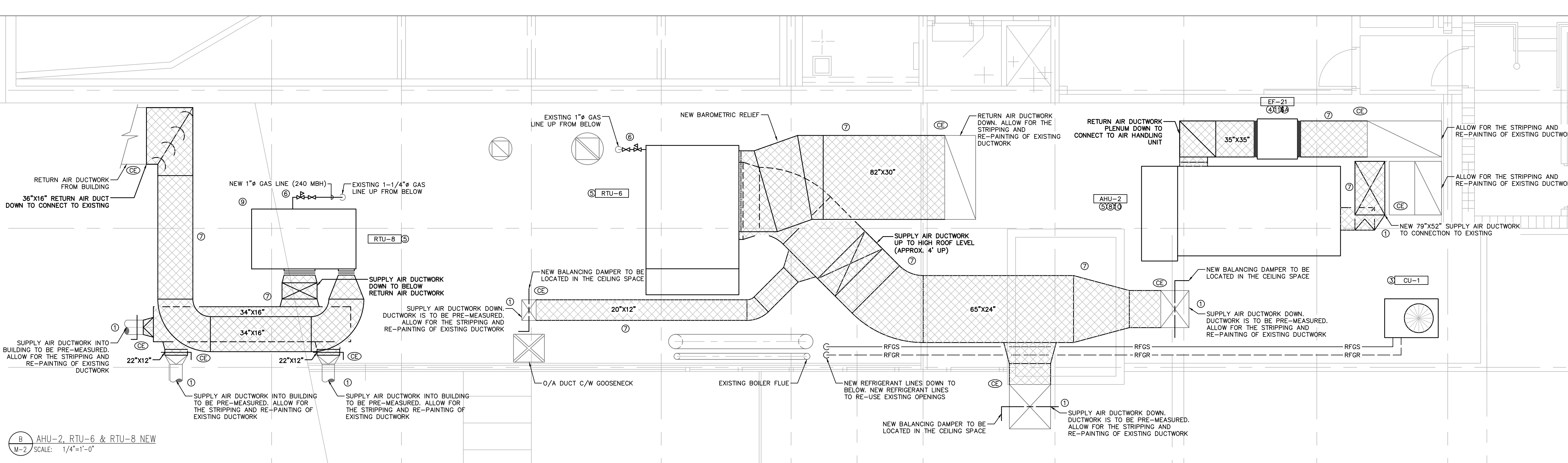
A AHU-2, RTU-6 & RTU-8 DEMO SCALE: 1/4"=1'-0"
