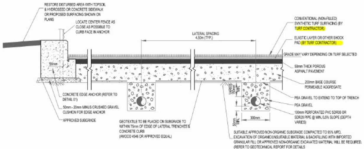
02 SYNTHETIC TURF FIELD WITH SHOCK PAD
